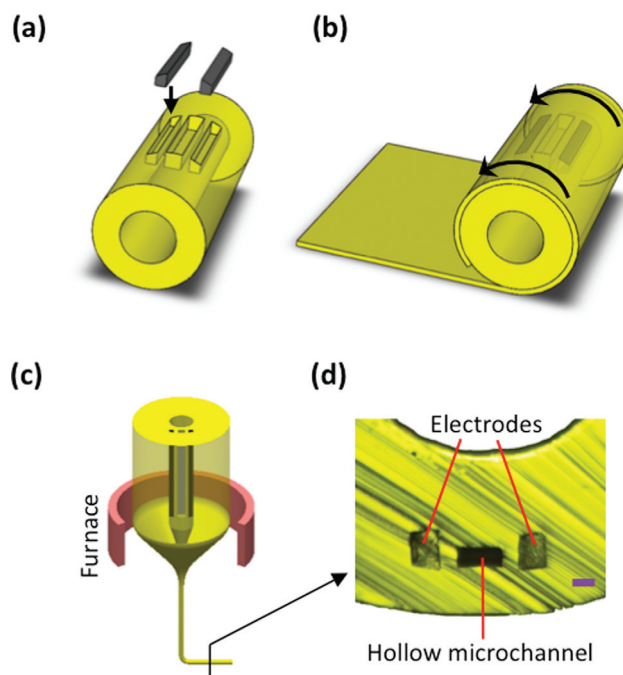
FIG. 1. Fiber fabrication. (a)–(c) Fabrication process flow and (d) Optical micrograph of the fiber structure containing a hollow microchannel flanked by conducting electrodes. Scale bar in (d) is 20 \mu\text{m} .
